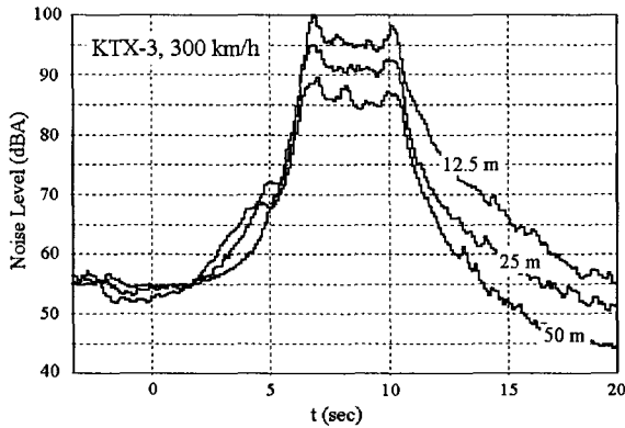
Figure 4. Time history of noise level of high speed train traveling at 300 km/h
