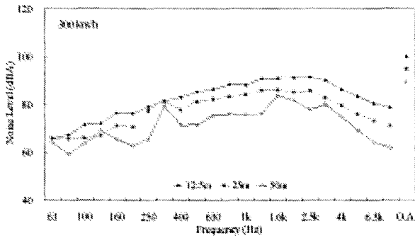
Figure 5. Pass-by noise spectra of high speed train running at 300 km/h
