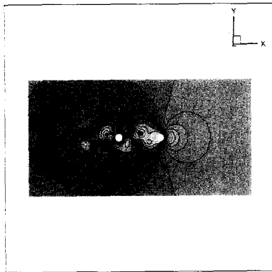
Fig.11 The pressure distributions at 5D ( Ut/D=200 )
