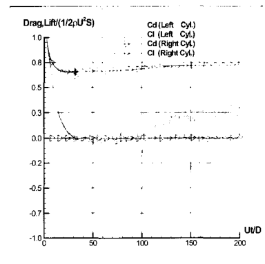
Fig.8 The drag and lift coefficients at 5D
