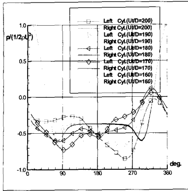
Fig.9 The pressure distributions along the cylinder surface at 5D
