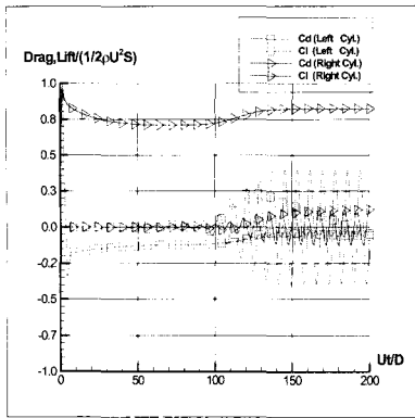
Fig.3 The drag and lift coefficients at 1D
