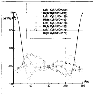
Fig.4 The pressure distributions along the cylinder surface at 1D
