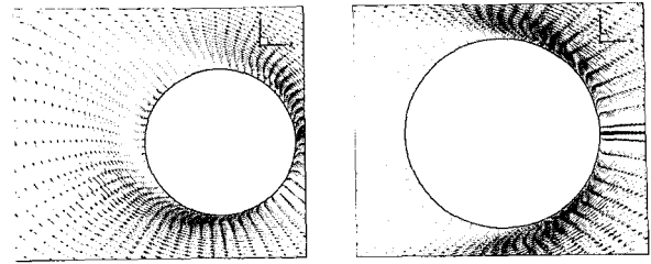
Fig.12 The velocity distributions at 5D ( Ut/D=200 )
