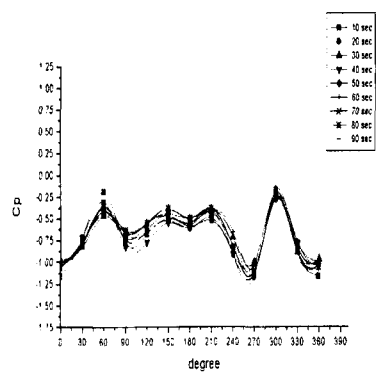
Fig.5 The pressure distributions along the cylinder surface at 1D
