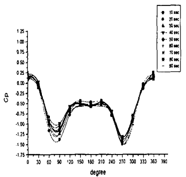
Fig10 The pressure distributions along the cylinder surface at 5D
