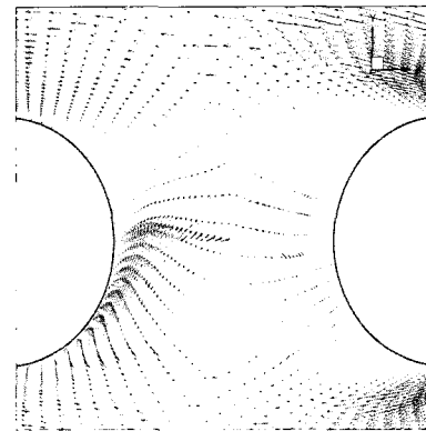
Fig.7 The velocity distributions at 1D ( U_t/D=200 )
