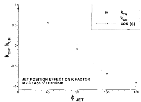
Fig.6 Jet effectiveness factor, k vs jet position angle
