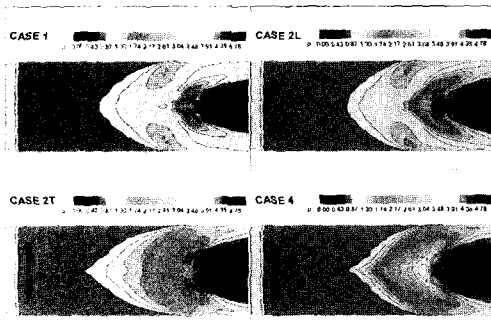
Fig.7 Surface pressure distributions near jet exit region for multiple jet activated cases
