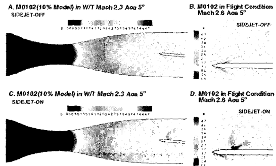
Fig.3 Pressure contours for 4 cases
