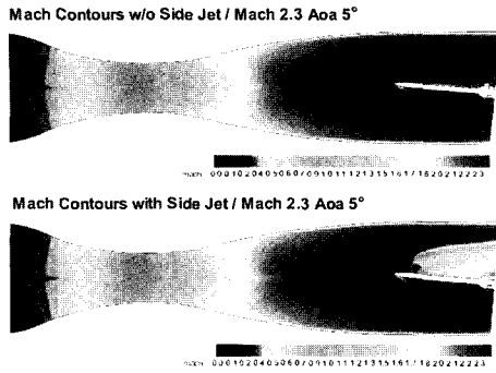
Fig.4 Mach contours for 10% Model with/without side jet
