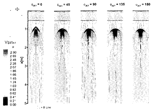
Fig.5 Unfold surface pressure contour for various jet positions
