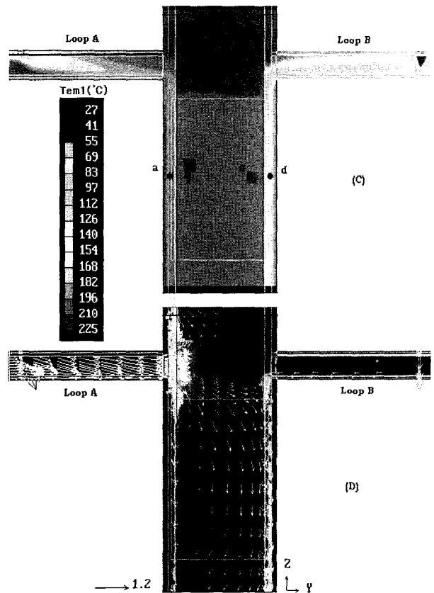
Fig. 5 Temp. (C) and vector (D) distribution of partial loop stagnation (Case 4)
