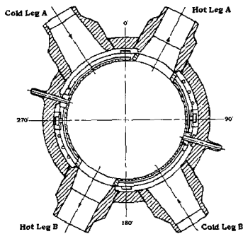
Fig. 1 Top View of RPV
