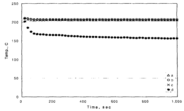
Fig. 9 Temp. comparisons of vessel downcomer for partial loop stagnation (Case 4)
