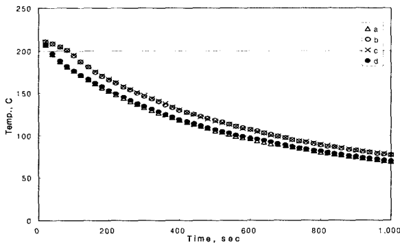
Fig. 6 Temp. comparisons of vessel downcomer for total loop stagnation (Case 1)
