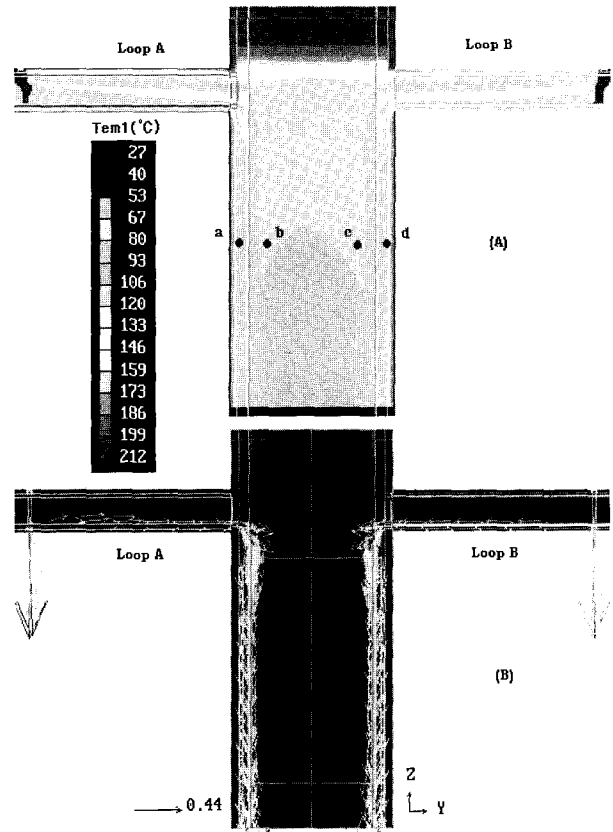
Fig. 4 Temp. (A) and vector (B) distribution of total loop stagnation (Case 1)
