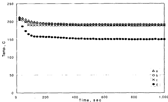
Fig. 7 Temp. comparisons of vessel downcomer for partial loop stagnation (Case 2)
