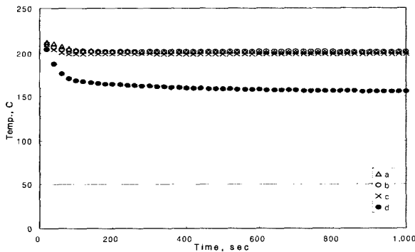
Fig. 8 Temp. comparisons of vessel downcomer for partial loop stagnation (Case 3)
