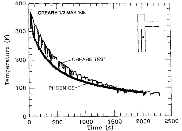
Fig. 3 Comparison of Temp. under Cold Leg
