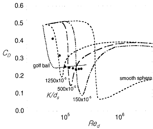
Figure 3. Variations of the drag coefficient due to active and passive devices as a function of the Reynolds number: circle, present study; dimples, [7]; roughness, [6].
