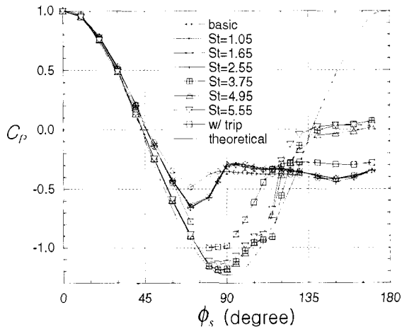
Figure 4. Static-pressure distribution on the sphere surface.
