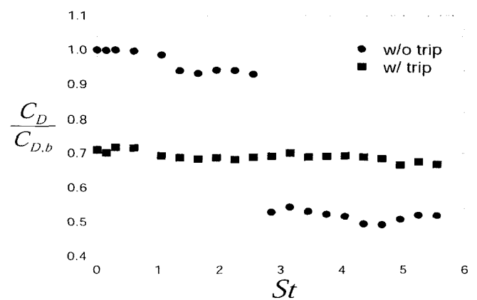
Figure 2. Variation of the drag coefficient with the forcing frequency.
