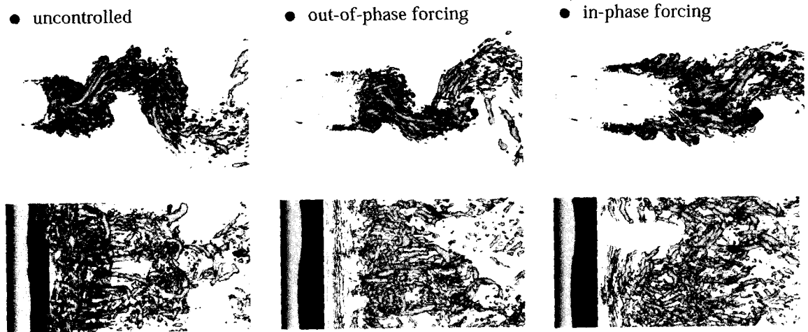
Figure 11. Changes in the instantaneous vortical structures due to the distributed forcing at Re=3900 .
