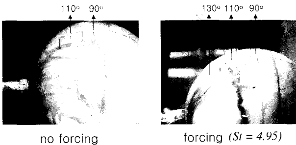
Figure 5. Oil flow pattern on the sphere surface.
