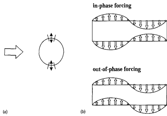
Figure 6. Schematic diagram of the distributed forcing: (a) side view; (b) front view.
