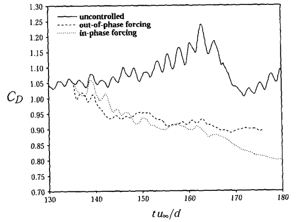
Figure 10. Variation of the drag coefficient due to the distributed forcing at Re=3900 .
