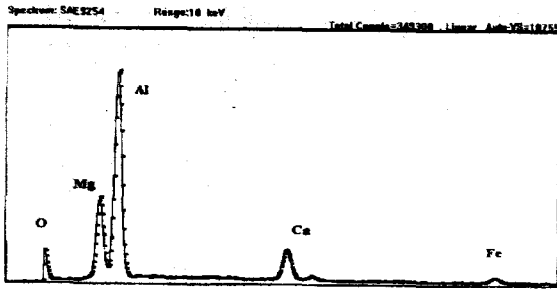
Fig. 23 Spectrometer pattern of nonmetal in fracture surface (SAE 9254)
