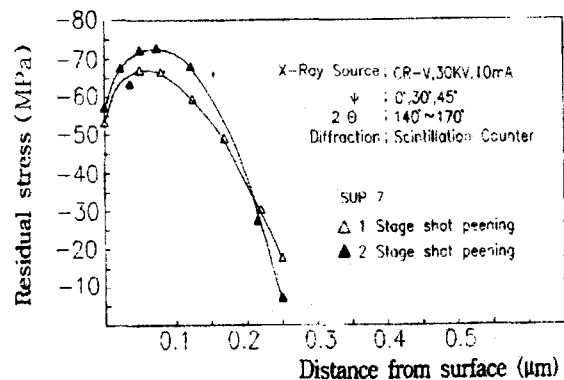
Fig. 6 Residual stress distributions produced by Shot-peening (50CrV4)
