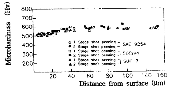
Fig. 10 Hardness distributions produced by Shot-peening(SAE 9254, 50CrV4, SUP 7)
