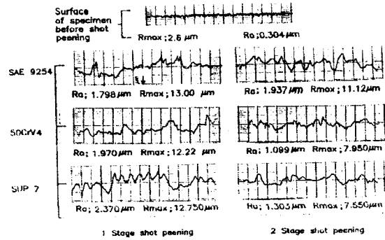
Fig. 9 Roughness pattern of shot peened specimen
