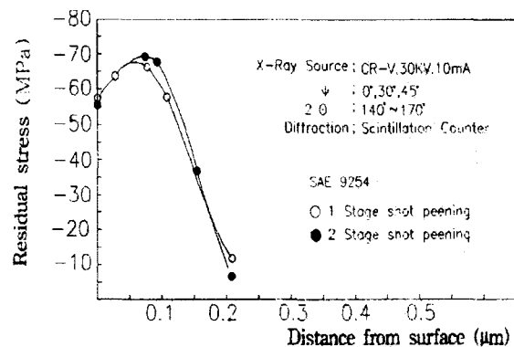
Fig. 5 Residual stress distributions produced by Shot-peening (SAE 9254)
