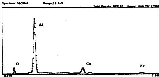
Fig. 24 Spectrometer pattern of nonmetal in fracture surface (50CrV4)
