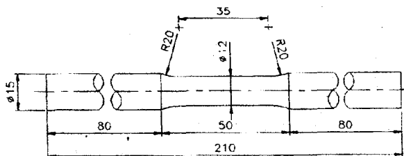
Fig. 1 Dimensions of Specimen
