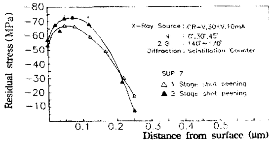
Fig. 7 Residual stress distributions produced by Shot-peening (SUP 7)
