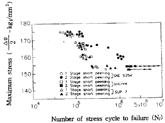
Fig. 14 Rotary bending fatigue S-N curves for SAE 9254, 50CrV4, SUP 7 specimen
