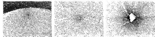
Specimen : DIN 50CrV4 Condition : 2段 Shot-Peening Fatigue Limit : \Delta\sigma/2 : 1660\text{MPa} ( \pm 830\text{MPa} ) Number of Cycles : 77,600 r.p.m. Fig. 22 SEM photographs of fish eye (nonmetal) fracture region under \Delta\sigma/2 = 1660\text{MPa}
