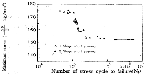
Fig. 13 Rotary bending fatigue S-N curves for SUP 7 specimen
