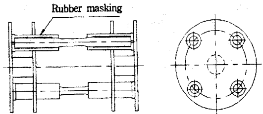
Fig. 2 Fixture of Specimen
