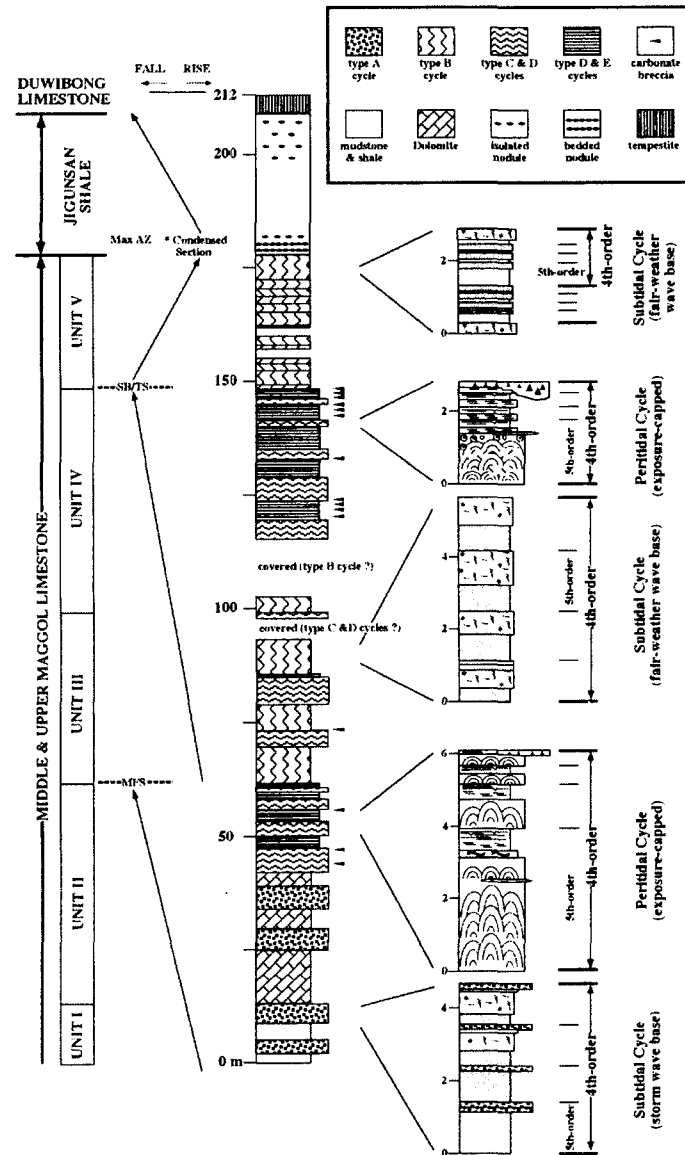
Fig. 4. Simplified columnar section of the middle and upper Maggol Limestone and the overlying Jigunsan Shale at Dongjeom area. On the basis of the systematic changes in stacking pattern of meter-scale fourth-order cycles, the middle and upper Maggol Limestone can be subdivided into five distinct units (I to V). Two third-order shallowing-upward cycles are recognized in the units I to IV. The overlying unit V is a stack of subtidal fourth-order cycles. Each boundary of third-order cycles represents a major marine-flooding surface. However, the boundary between units IV and V is a sequence boundary as well as transgressive surface. Note the 4:1 bundling of fifth-order cycles within fourth-order cycles. Abbreviations: MFS = major marine-flooding surface; Max AZ = Maximum Accommodation Zone; SB/TS = sequence boundary/transgressive surface.
