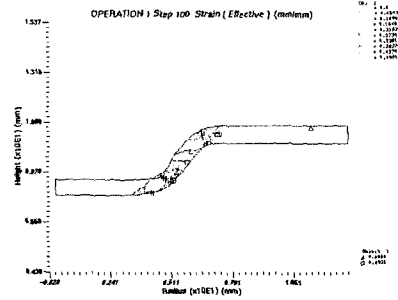
(a) Strain deformation of 1st-drawing
