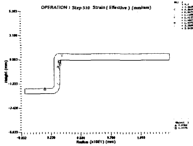
(e) Strain deformation of 5th-drawing
