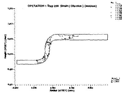
(b) Strain deformation of 2nd-drawing
