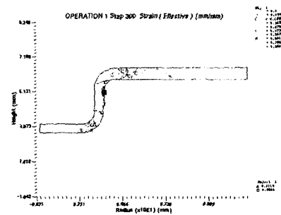
(c) Strain deformation of 3rd-drawing
