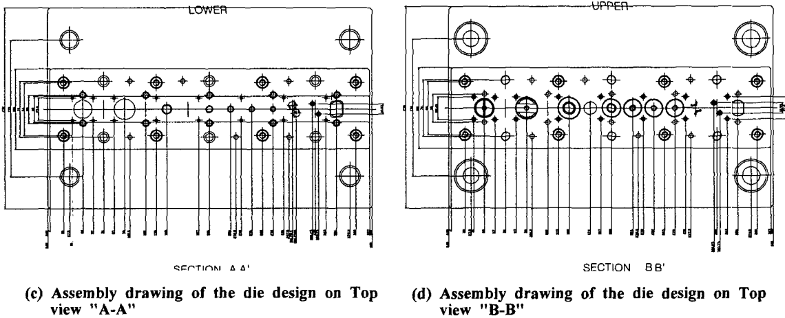
Fig. 7 Die assembling drawing
