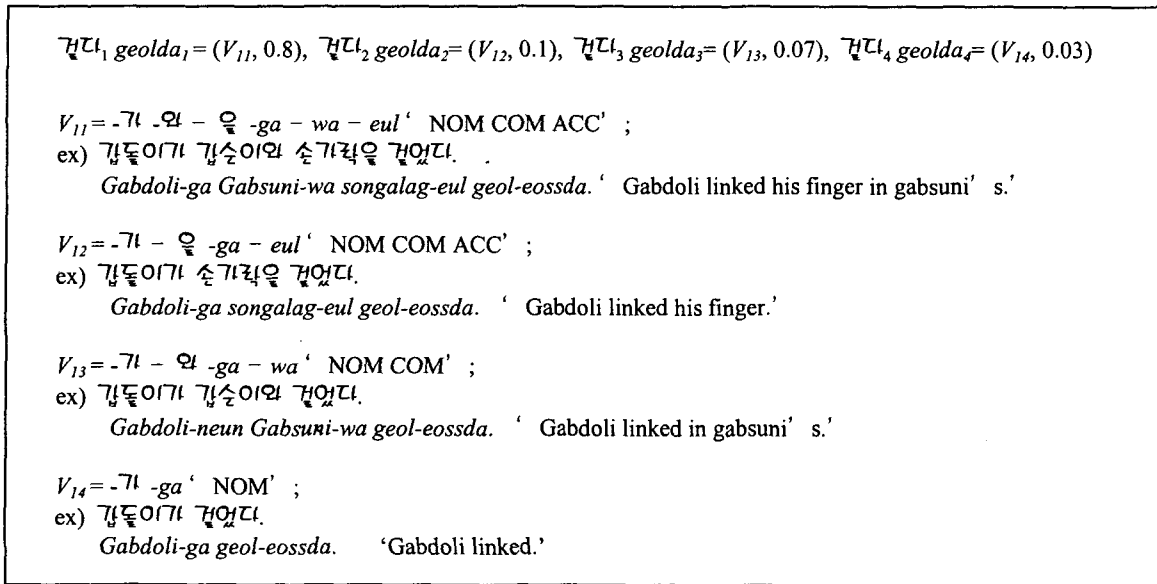
Figure 4. Examples of the probabilistic Case structures of the verb 걸다 geolda 'link'
