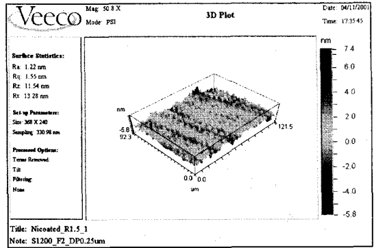
Fig. 4 Roughness(Ra:nm) of Ni 2 coated
