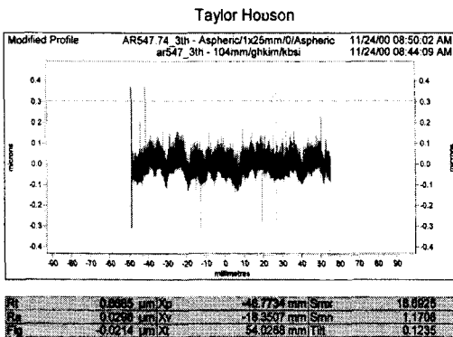
Fig. 8 Measure of Aspheric Ni reflector by Form Talysurf
