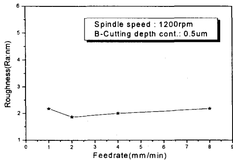
(b) Feedrate
