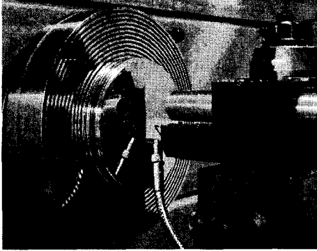
Fig. 5 Manufacture of Aspheric Ni_coated mirror
