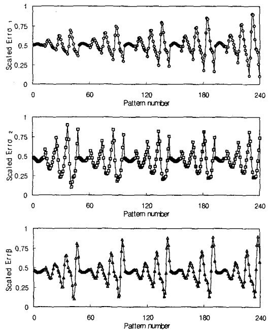
Fig. 7 Scaled target value for minus stress ratio
