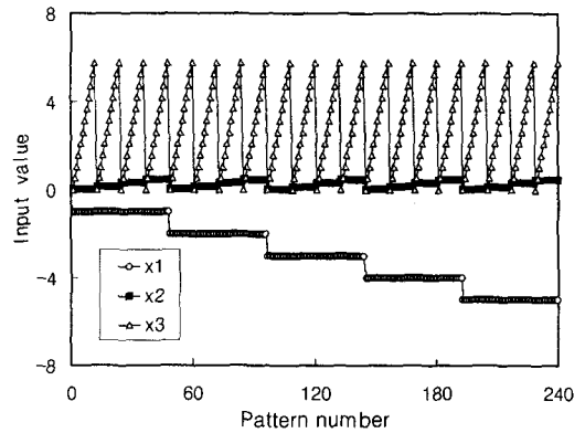
Fig. 6 Input value for minus stress ratio
