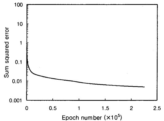
Fig. 8 Sum squared error according to the epoch number for minus stress ratio
