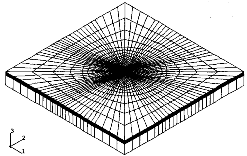
Fig. 4 3-Dimensional finite element model
