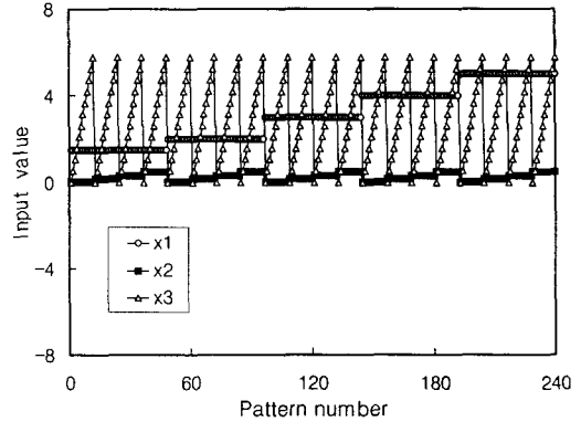
Fig. 10 Input value for plus stress ratio
