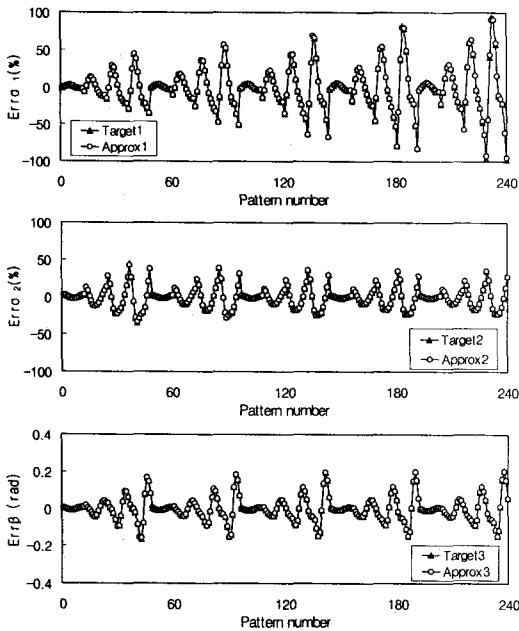
Fig. 9 Comparison network output value with target one for minus stress ratio
