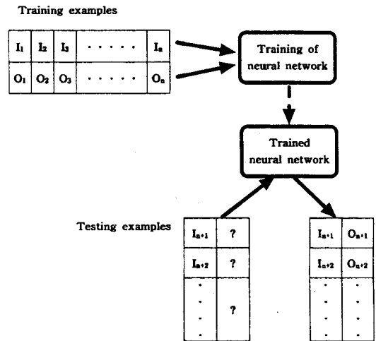
Fig. 1 Generalization procedure of neural network
