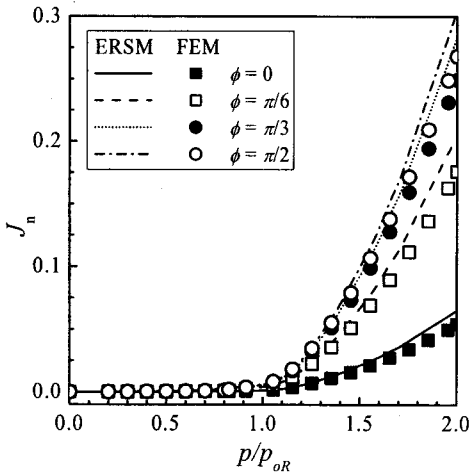
Fig. 6 Comparison of the FE J results at various points along the crack front ( \phi=0, \pi/6, \pi/3 and \pi/2 ) with those estimated from the proposed ERSM for global bending: TP 316 with a/t=0.2 and \beta/\pi=0.1 .
