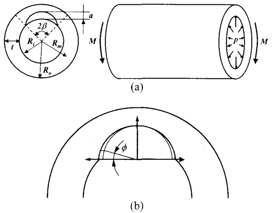
Fig. 1 (a) Schematic illustration for surface cracked pipes in internal pressure p and in global bending M , and (b) definition of the crack angle \phi .
