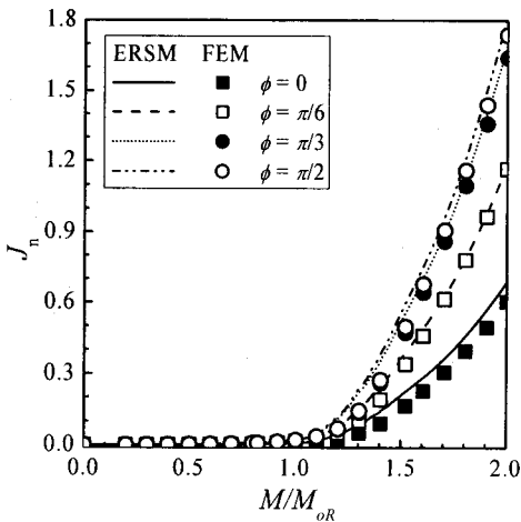
Fig. 7 Comparison of the FE J results at various points along the crack front ( \phi=0, \pi/6, \pi/3 and \pi/2 ) with those estimated from the proposed ERSM for global bending: TP 304 with a/t=0.5 and \beta/\pi=0.1 .
