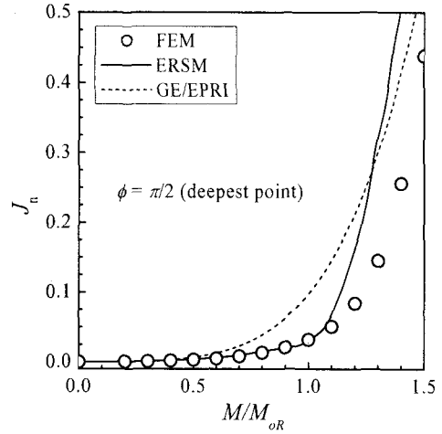
Fig. 5 Comparison of the FE J results with those estimated from the proposed ERSM and from the GE/EPRI method for the TP304 material under global bending: a/t=0.5 , \beta/\pi=0.4 .
