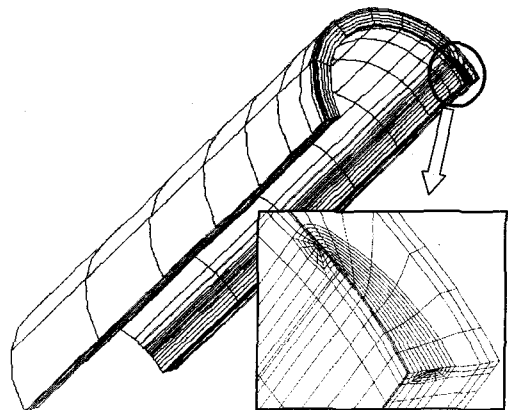
Fig. 3 A typical FE mesh for R_m/t=5 , a/t=0.3 and \beta/\pi=0.1 .
