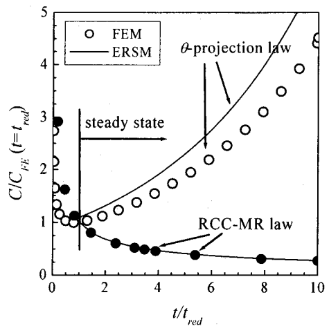
Fig. 8 Comparison of the FE C^* results with those estimated from the proposed ERSM for internal pressure with a/t=0.5 and \beta/\pi=0.4
