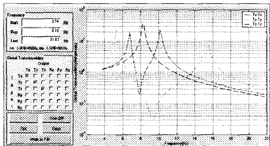
Fig.4 Force Transmissibility of Mount System
