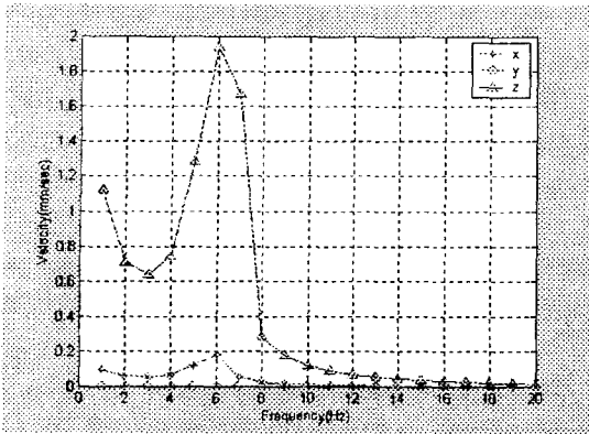
Fig.10 Velocity under Mount due to Base Motion
