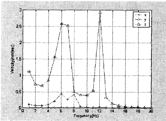
Fig.11 Vibration Response Due to Base Motion after Optimization
