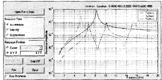
Fig.6 Vibration Response of Mount System due to Internal Force
