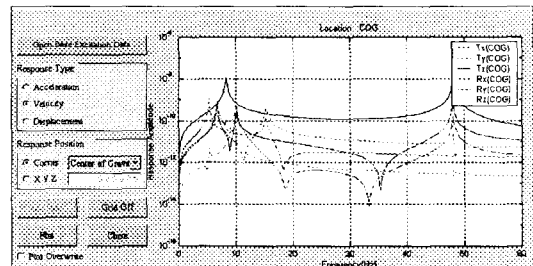
Fig.7 Vibration Response of Mount System due to External Base motion
