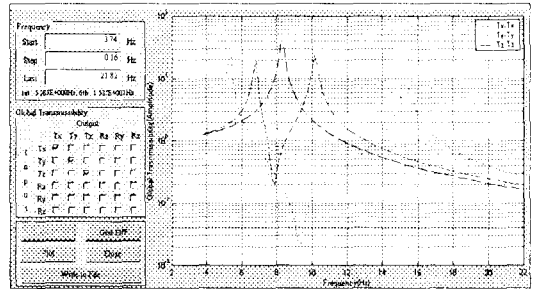
Fig.5 Motion Transmissibility of Mount System
