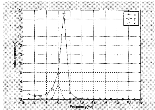
Fig.9 Vibration Response Due to Base Motion before Optimization
