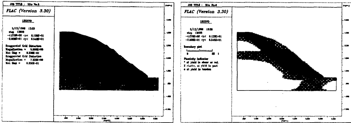
Figure 4. The result of FLAC
