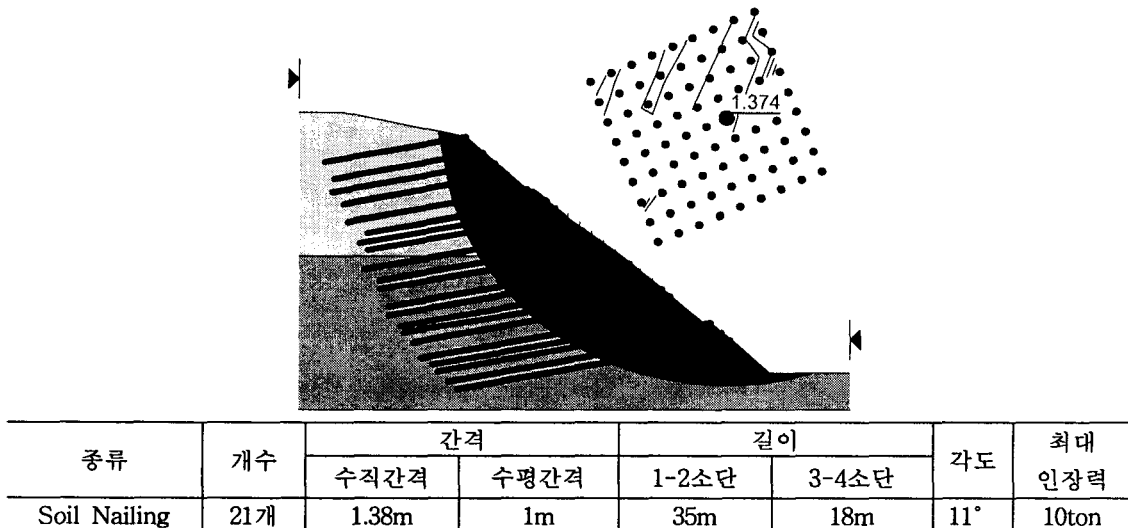
Figure 5. Soil Nailing reinforcement
