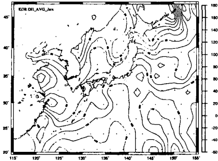
Fig. 2. Mean sea level in centimeters in the East Asian Marginal Seas from the 7 years of T/P measurements.
