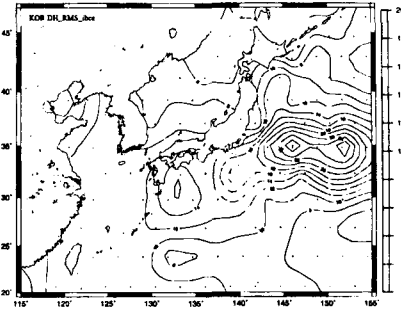
Fig. 3. Sea level variability in centimeters in the East Asian Marginal Seas from the 7 years of T/P measurements.
