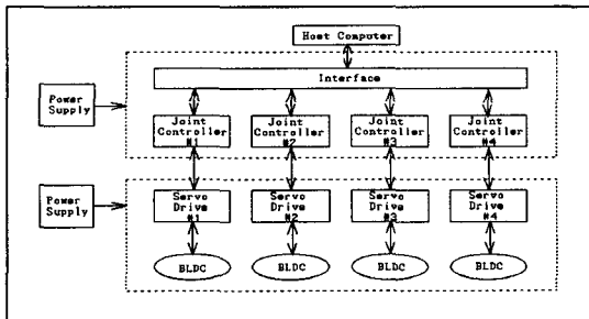
Fig. 2 Overall system block diagram.
