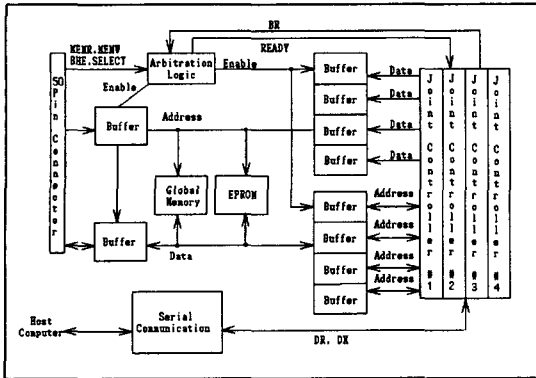
Fig. 4 Interface block diagram.
