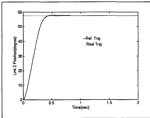
Fig. 9 Position tracking performance of 2 link with 1 radian under payload(2kg).
