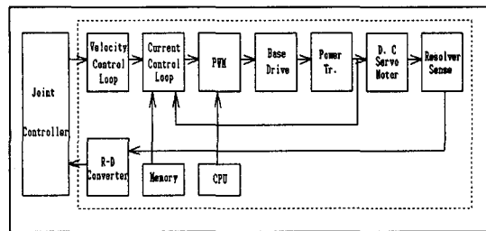
Fig. 3 AC servo drive.
