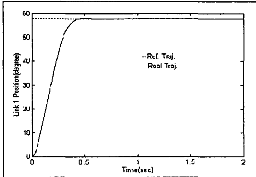
Fig. 7 Position tracking performance of 1link with 1 radian input under payload(2kg)
