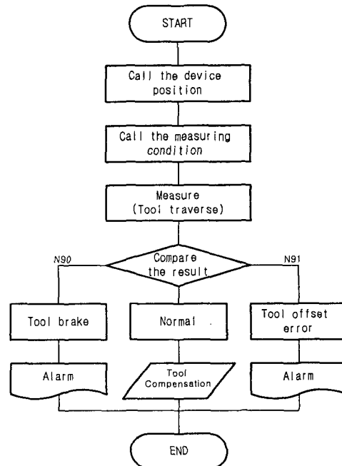
Fig. 6 Flow chart of macro program
