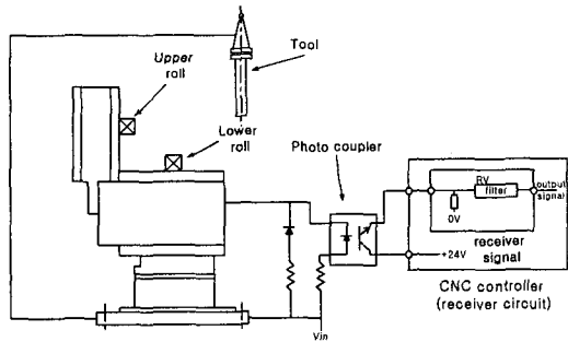
Fig. 4 Schematic diagram of the measuring device
