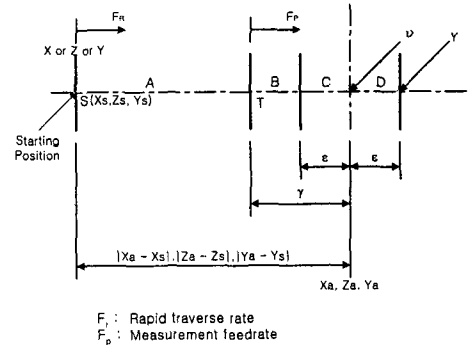
Fig. 5 Predicated measurement position
