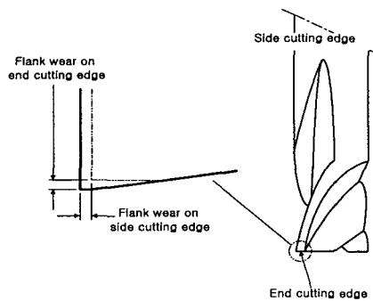
Fig. 1 Flank wear of milling tool
