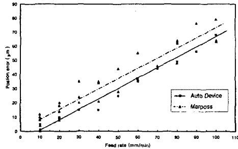
Fig. 8 Setting position error comparison between marposs device and developed device
