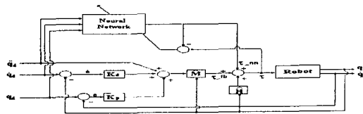
Fig. 2 The block diagram of proposed neural control Structure for robot manipulator
