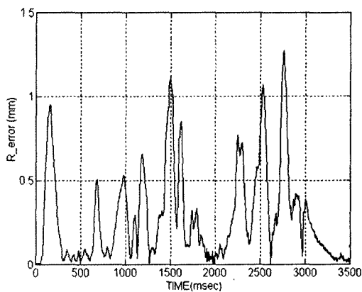
Fig. 11. Tracking error of existing controller(PID) with 2.0 kg payload.
