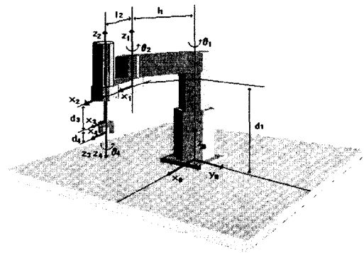
Fig. 3. Coordinates frame of SCARA robot.
