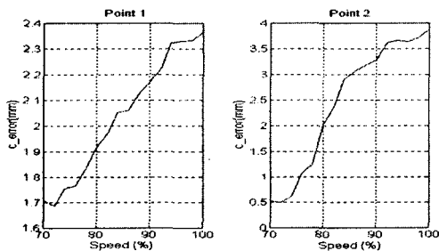
Fig. 14. Experimental results of existing controller(PID) for repeating precision at cartesian coordinates.
