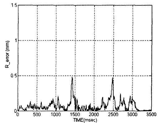
Fig. 10. Tracking error of neural controller with 2.0 kg payload.
