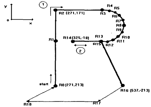
Fig. 9. Reference trajectory at cartesian coordinates.
