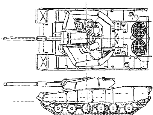
Fig.1 External of Track Vehicle
