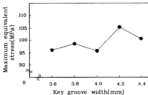
Fig. 11 Stress value according to change of key groove width
