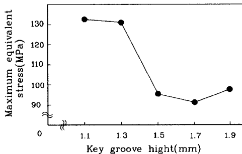
Fig. 10 Stress value according to change of key groove height
