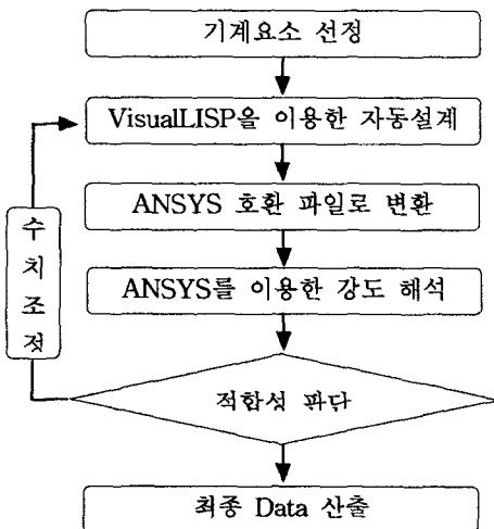
Fig. 4 Algorithm of optimum design using ADS and FEA
