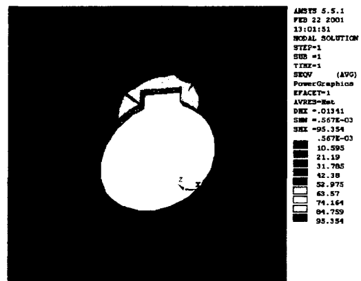
Fig. 9 Distributed equivalent stress when key width is 4 mm & key height is 1.5 mm
