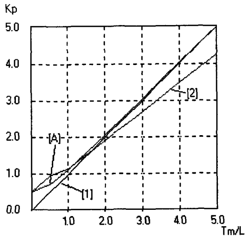
Fig.2 Gains by methods of Z-N[1], Z-N[2] and Approx. Formula [A] at P control ( K_m=1.0 , L=0.5[\text{min}] )
