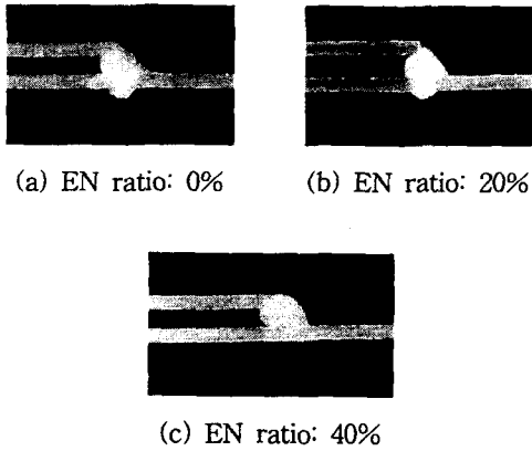
Fig. 6 Macro-section as various EN ratio in Al 5052 lap joint (root gap: 1.5mm, 100cm/min, 70A, 15V )
