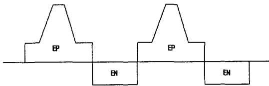
Fig. 1 EP and EN of AC pulse Welding
