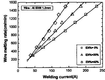
Fig. 2 Relationship between EN ratio and wire melting rate (MIG) [1]
