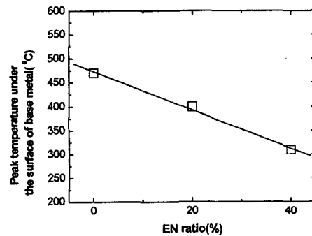
Fig. 3 Heat input by EN ratio (6mm from the center line of bead) [1]
