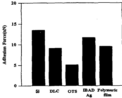
Fig. 9 Adhesion forces of different hydrophobic surfaces.
