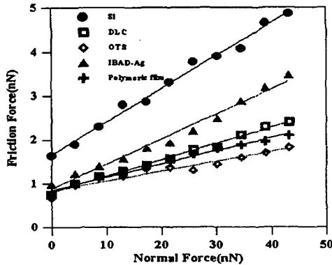
Fig. 10 Friction forces of different hydrophobic surfaces with the normal load.
