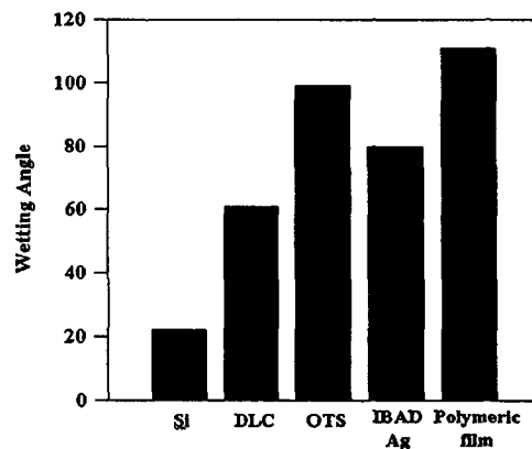
Fig. 8 Wetting angles of different hydrophobic surfaces.
