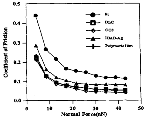
Fig. 11 Coefficient of friction of different hydrophobic surfaces with the normal load.
