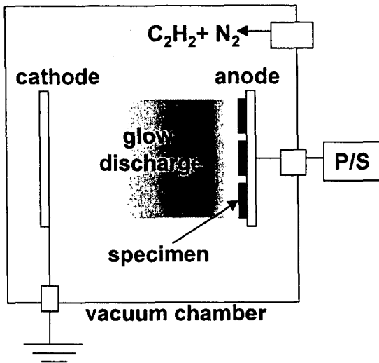
Fig. 1 A schematic view of plasma surface modification
