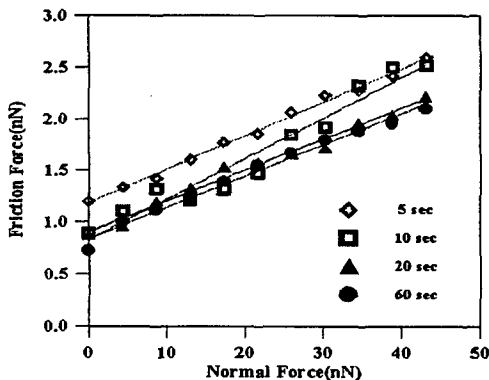
Fig. 7 Friction forces of different plasma treating time specimens with the normal load.
