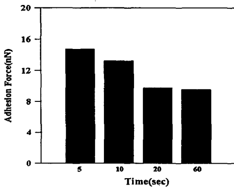
Fig. 6 Adhesion forces with the plasma treating time.
