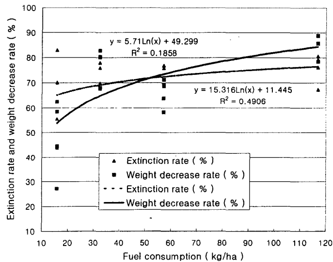
Fig 2. Weed extinction rate and weight decrease rate by fuel consumption.
