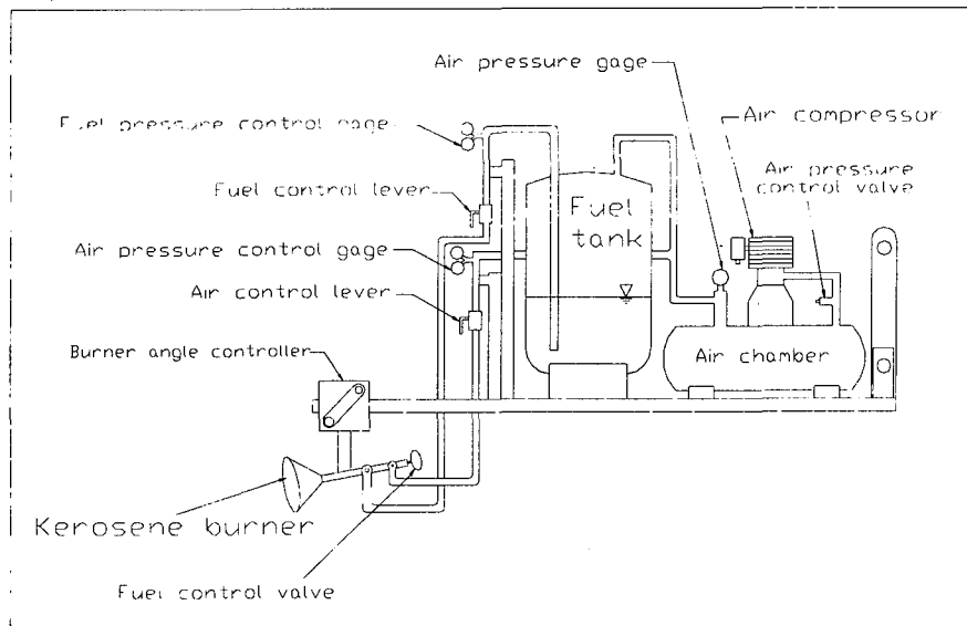
Fig. 1 Side view of kerosene flame weeder.
