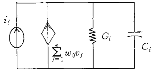
Fig. 2. The Equivalent circuit seen from input node i.
