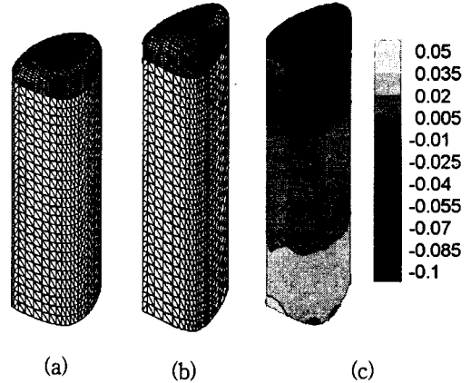
Fig. 5 (a) Initial guess generated by the direct mesh mapping (stage 5); (b) Final shape generated by the direct mesh mapping (stage 6); (c) Calculated thickness strain distribution of stage 6
