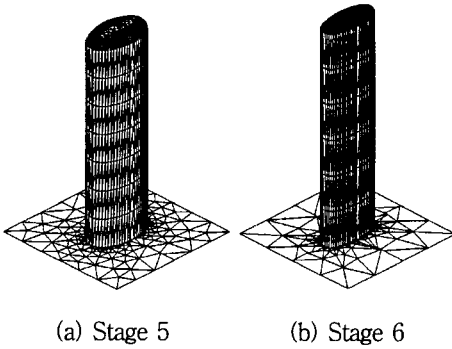
Fig. 3 Sliding constraint surfaces for the multi-stage inverse analysis of rectangular cup drawing process with large aspect ratio
