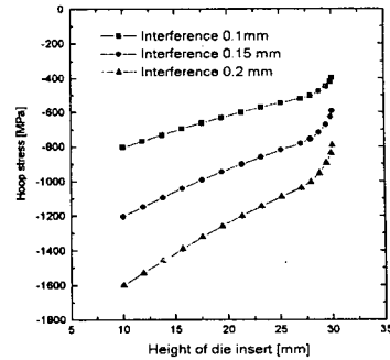
Fig. 4 Hoop stresses of the die insert with interference values
