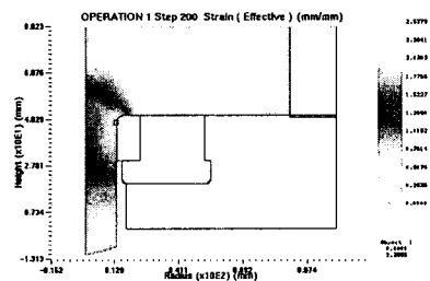
Fig. 2 Effective strain distribution of the hot extrusion
