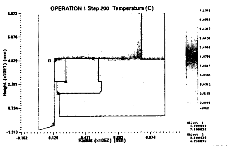
Fig. 3 Temperature distribution on the die insert and case
