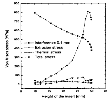
Fig. 5 Equivalent stresses on the height of die insert due to mechanical and thermal loads
