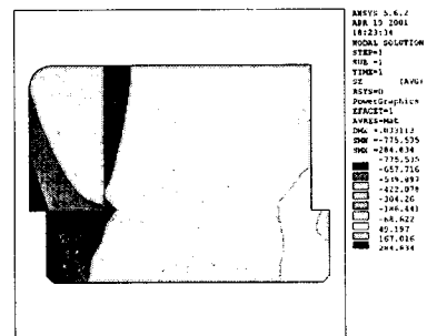
Fig. 6 Hoop stresses on the height of die insert due to mechanical and thermal loads
