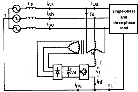
Fig 2. Active neutral harmonic suppressor system
