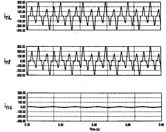
Fig 4. Simulated waveforms of the conventional control method
