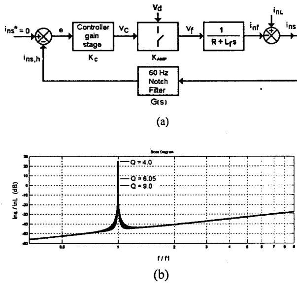
Fig 3. Block diagram and compensation characteristics of the conventional control method. : (a) block diagram of the closed loop control system and (b) compensation characteristics
