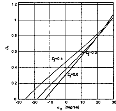
Fig. 7. Control range of \alpha_2 .
