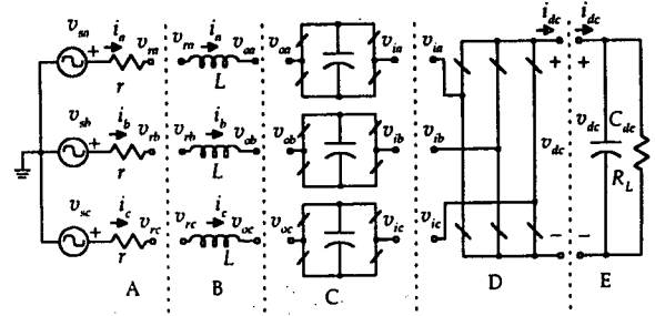
Fig. 3. Circuit partitioning.
