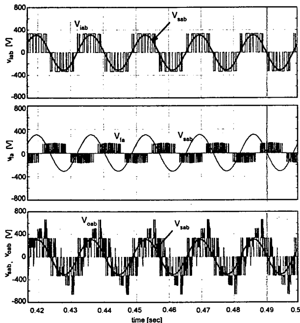
Fig. 11. Switching waveforms; (upper) line-to-line voltage of TP inverter, (middle) line-to-line voltage of FB inverter, (lower) the resultant 9-level line-to-line output voltage of the multilevel PWM rectifier.
