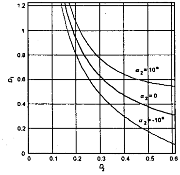
Fig. 6. Control range of D_1 and D_2 .
