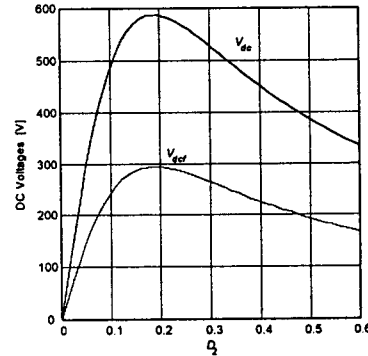
Fig. 9. Variation of V_{dc} and V_{def} with respect to D_2 .
