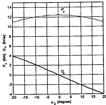
Fig. 8. P_s and Q_s with respect to \alpha_2 .
