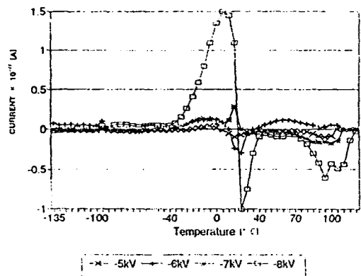
Fig. 6. TSC Spectra according to Forming Electric Field
