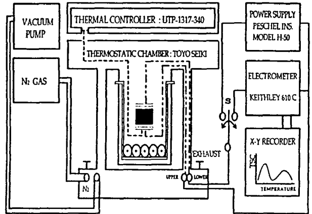
Fig. 3. Schematic Drawing of TSC Experimental Device
