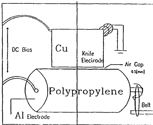
Fig. 2. Corona Charging Device
