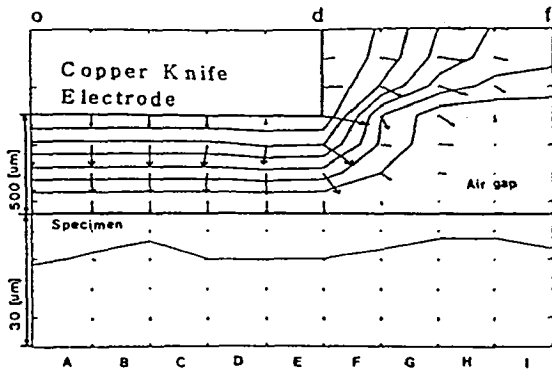
Fig. 7. Electrostatic Contour and Electric Field Distribution (→: Electric Field)
