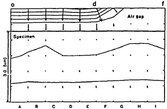
Fig. 9. Electrostatic Contour and Electric Field Distribution inside Specimen (→: Electric Field)
