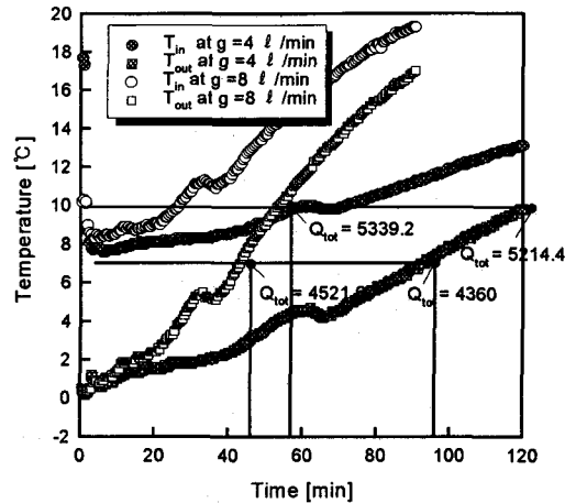
Fig. 7 Variation of inlet-outlet temperature in storage tank.
