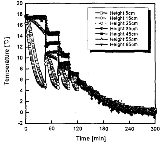
Fig. 4 Transient water temperature response of ice storage tank( T_{ei} : -4^{\circ}\text{C} ).
