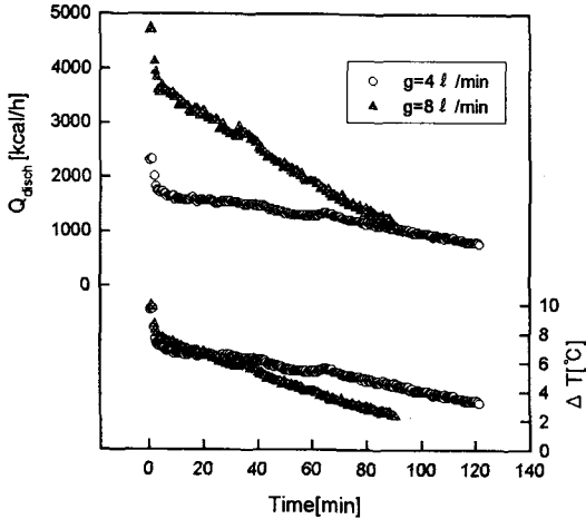
Fig. 8 Variation of discharging rate in storage tank.
