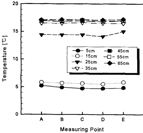
Fig. 3 Horizontal water temperature distribution in storage tank( T_{ei} : -4^{\circ}\text{C} , Time : 40min).
