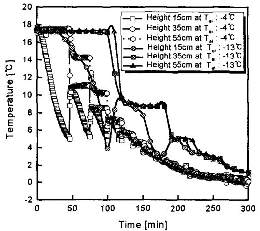
Fig. 5 Transient water temperature response of ice storage tank( T_{ei} : -4^{\circ}\text{C} , -13^{\circ}\text{C} ).
