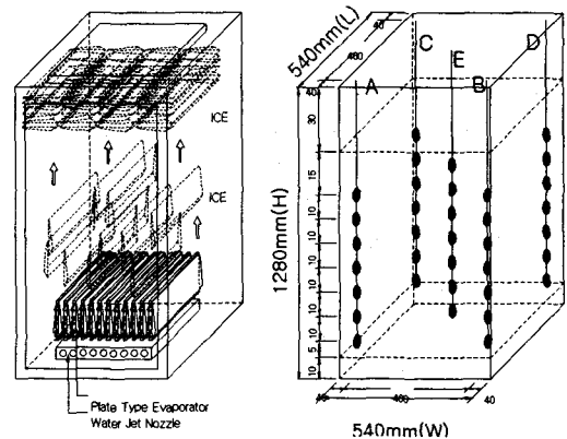
Fig. 2 Schematic diagram of ice storage tank.
