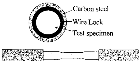
Fig. 4 Fatigue test specimen with Wire Lock
