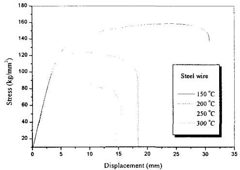
Fig. 3 Tensile properties of high temperature
