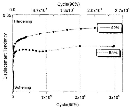
Fig. 9 Relation between displacement and cyclic number
