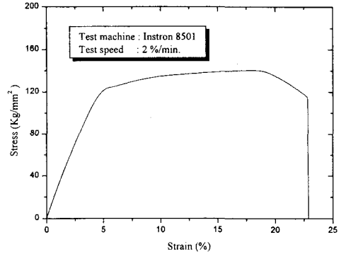
Fig. 2 Tensile property of steel wire
