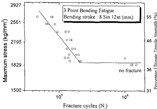
Fig. 13 S-N diagram by 3 points bending fatigue test for steel wire
