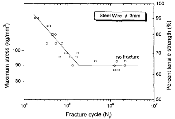
Fig. 8 S-N diagram for steel wire
