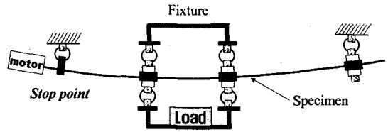
Fig. 5 Apparatus for Nakamura fatigue tester
