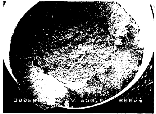
Fig. 10 Fatigue Fracture surface of steel wire
