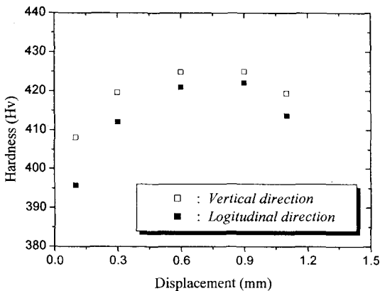
Fig. 7 Vickers Hardness with surface location
