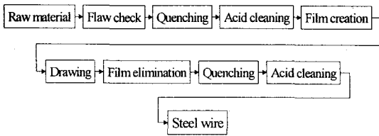
Fig. 1 Manufacturing process of steel wire
