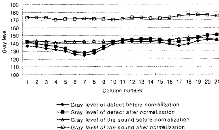
Fig. 4. Effect of image normalization on distribution of gray level.
