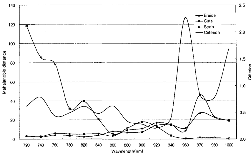
Fig. 3. Mahalanobis distance computed with the filter images of the sound and each defective part of Fuji apple in NIR range, and criteria for discrimination of the defectives from the sound.
