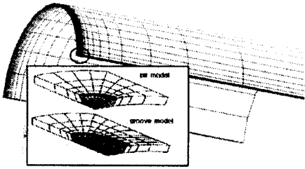
Fig. 1 Finite-element model on a semi-elliptical external corroded pipeline
