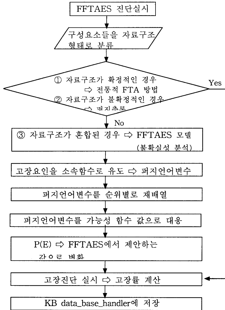
<Fig. 2> FFTAES flow chart
