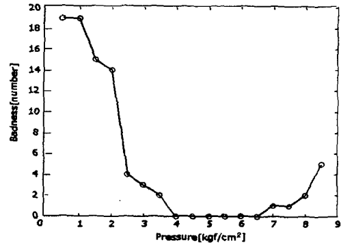
Fig. 7 The number of badness vs. the pressure variation
