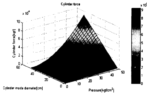
Fig. 2 Cylinder interior force according to the change of a cylinder inside diameter and pressure
