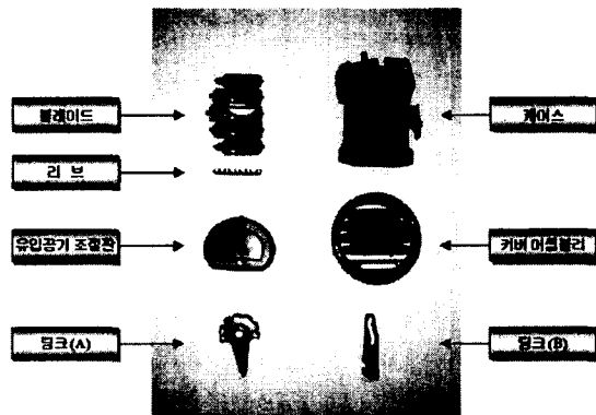
Fig. 4 Vent-grille parts
