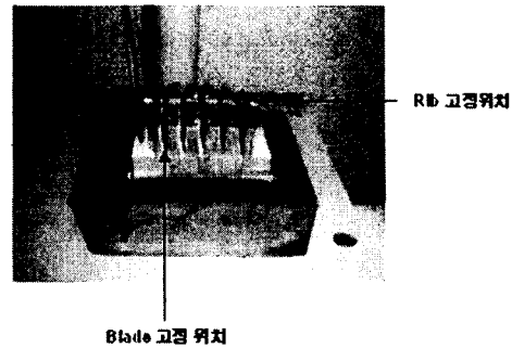
Fig. 3 A blade and rib setting jig
