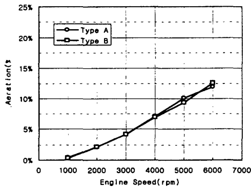
Fig.6 Effects of change of engine stroke on Aeration ( A_{O(ref)} ) with against engine rpm
