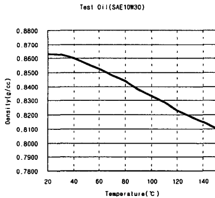
Fig.2 Variation of oil density with temperature
