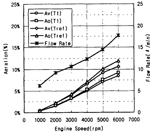
Fig.3 Variation of Aeration and oil flow rate at pump outlet with engine rpm. T_{oil}=90^{\circ}\text{C}
