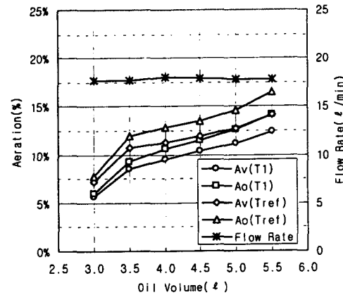
Fig.5 Variation of Aeration and oil flow rate at pump outlet with oil temperature at 6000 rpm
