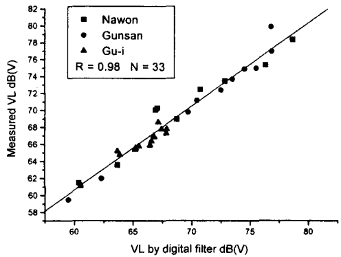
Fig. 7. Relationship between VL by digital filter and measured VL.
