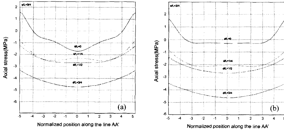
Fig. 6. Distribution patterns of \sigma_{xx} along the line AA' in Fig. 2 as a function of crack overlapping/crack length ratio ( d/L ) with fixing crack space/crack length ratio ( s/L ) to 3/4 . (a) before the onset of propagation, (b) after crack coalescence.
