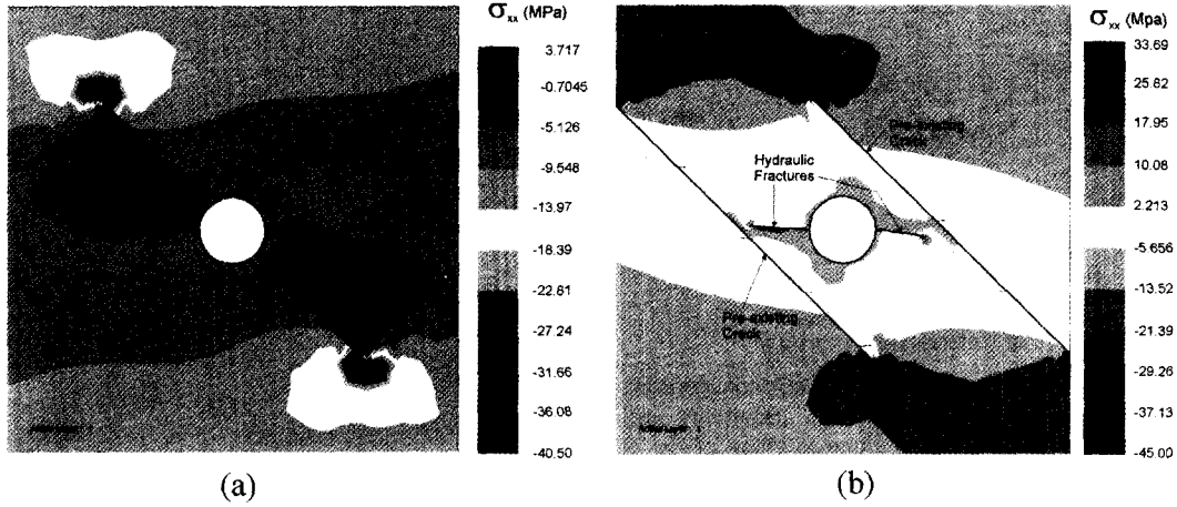
Fig. 11. Stress state transition after hydraulic fracture propagation. (a) One-crack configuration, (b) two-crack configuration. We can see the new-developed hydraulic fracture as well as the propagation of pre-existing crack, and the direction of hydraulic fractures is not exactly parallel to the direction of \sigma_{xx} .
