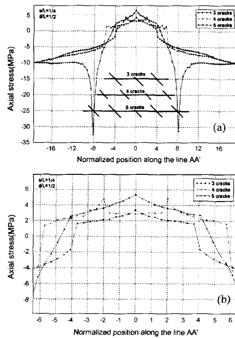
Fig. 8. Distribution patterns of \sigma_{xx} along the line AA' on several cases of crack quantity with fixing ratio of d/L=1/2 , s/L=1/4 . (a) before the onset of propagation for the whole length of model, (b) after crack coalescence for the x-range of crack location only.
