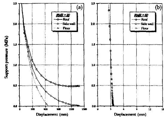
Fig. 2. Load-deformation characteristic curve from closed form solution. (a) RMR = 20, (b) RMR = 60
