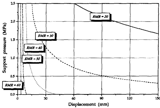
Fig. 3. Load-deformation characteristic curve nomogram. (closed form solution)
