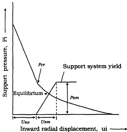
Fig. 1. Rock-support interaction curve.
