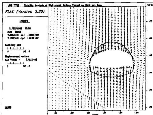
Fig. 7. Displacement vector of tunnel by back filling.
