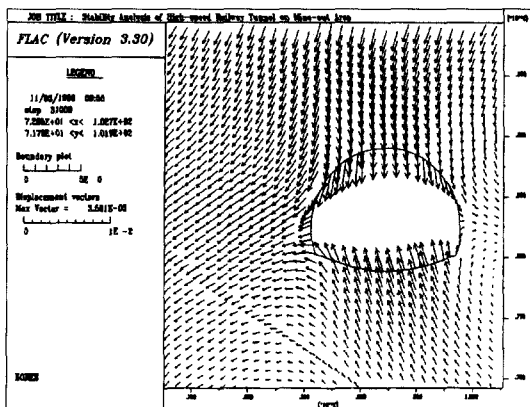
Fig. 5. Displacement vector of railroad tunnel.
