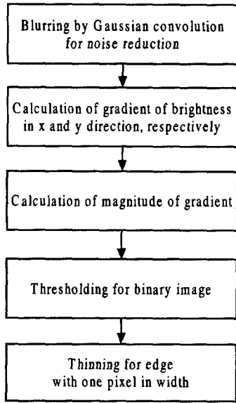
Fig. 8. Procedure for Canny edge detection.
