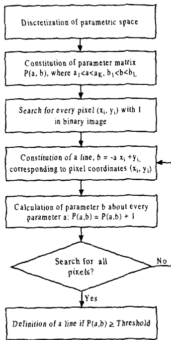
Fig. 10. Procedure for Hough transformation.
