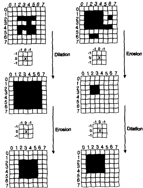
Fig. 11. Concepts of dilation and erosion. (a) A dilation-erosion scheme, (b) an erosion-dilation scheme.
