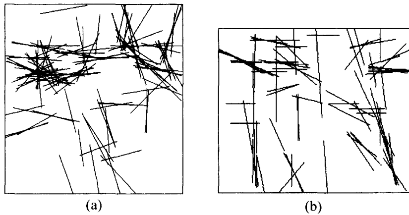
Fig. 19. Binary output images of Hough transform. (a) Gradient threshold = 14, Line threshold = 70, Hough threshold = 158, (b) Gradient threshold = 20, Line threshold = 40, Hough threshold = 180.
