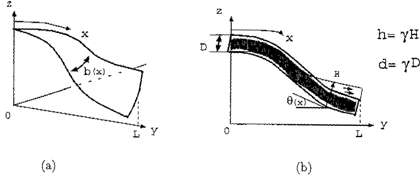
Figure 7: Schematic drawing of a flow model; (a) a quasi-three-dimensional shape of a slope element; (b) water flow movement on a slope element.
