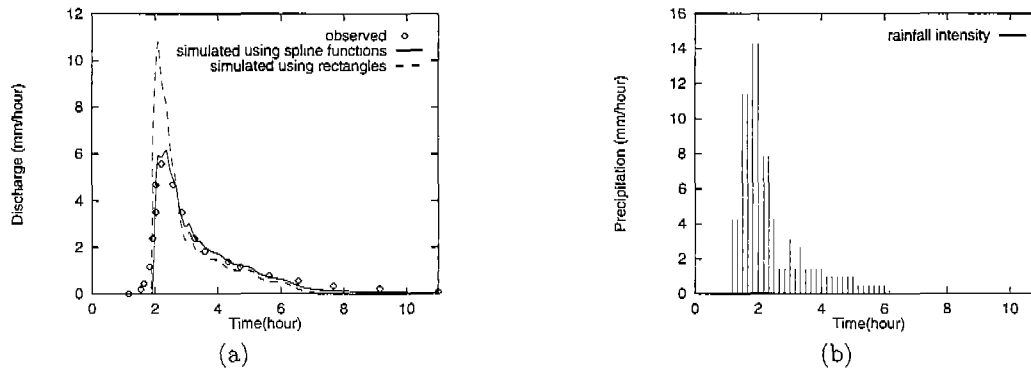
Figure 8: (a) Simulated and observed hydrographs. (b) Observed precipitation.
