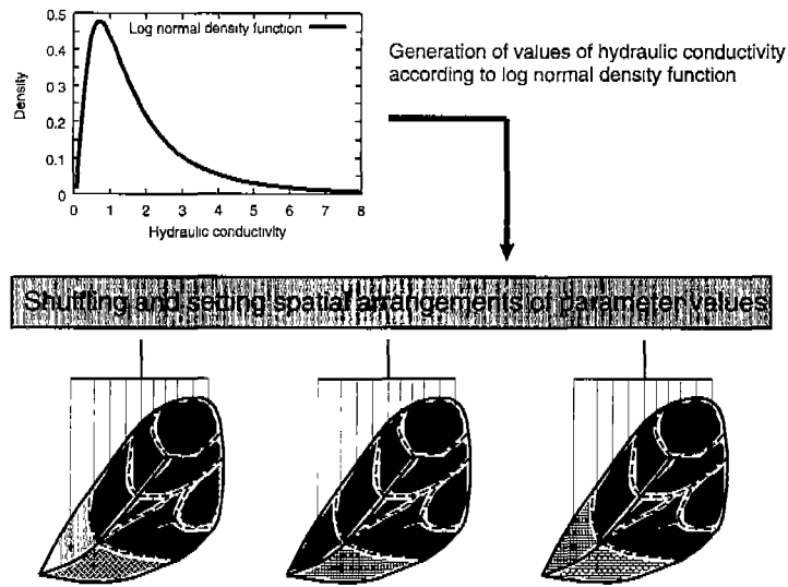
Figure 9: Simulation method.
