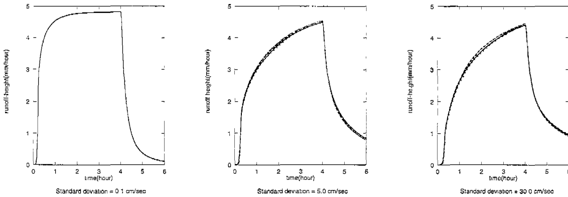
Figure 10: Comparison of simulated hydrographs. In each figure, five simulated hydrographs are drawn. On the five hydrographs, locations of assigned hydraulic conductivity values are different, but the values of mean and variance in the study area are same. In all cases, hydrographs are quite similar.
