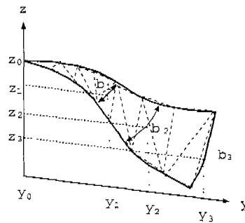
Figure 6: Approximation of a slope element by using cubic spline functions.
