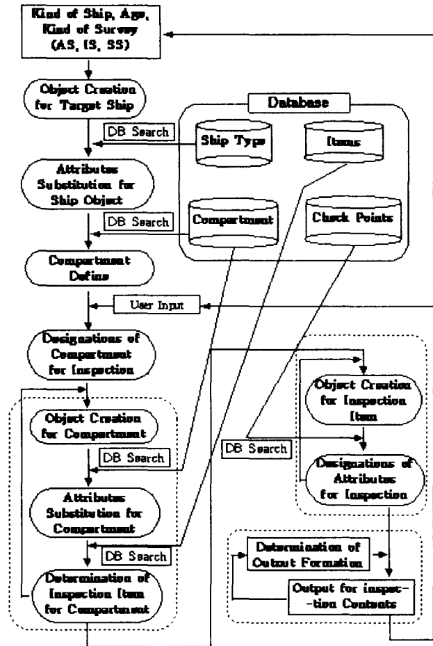
Fig. 4 Flow-chart of ship survey information system
