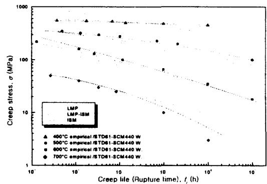
Fig. 11 Comparison of creep design curves for friction welded joints(STD61-SCM440) by ISM, those by LMP-ISM, LMP methods and the empirical data at 400, 500, 600 and 700°C
