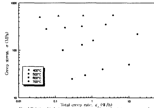
Fig. 4 Relationship between creep stress and total creep rate of STD61 to SCM440 at 400, 500, 600 and 700°C
