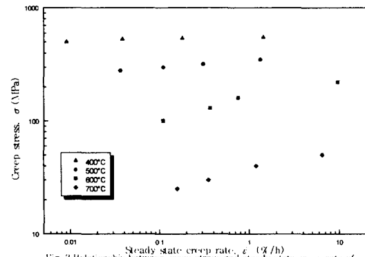
Fig. 3 Relationship between creep stress and steady state creep rate of STD61 to SCM440 at 400, 500, 600 and 700°C
