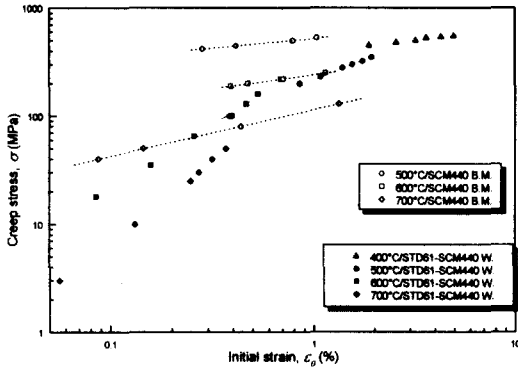
Fig. 8 Relationship between creep stress and initial strain for friction welded joints (STD61-SCM440) and SCM440 base metals at 400, 500, 600 and 700°C
