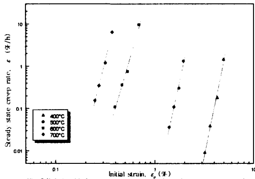
Fig. 5 Relationship between creep stress and steady state creep rate of STD61 to SCM440 at 400, 500, 600 and 700°C
