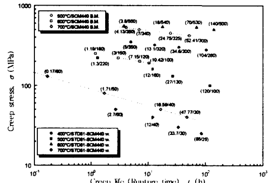
Fig. 7 Relationship between creep stress and creep life for friction welded joints (STD61-SCM440) and SCM440 base metals at 400, 500, 600 and 700°C
