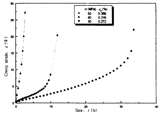
Fig. 2(d) Creep curves for friction welded joint (STD61-SCM440) at 700°C
