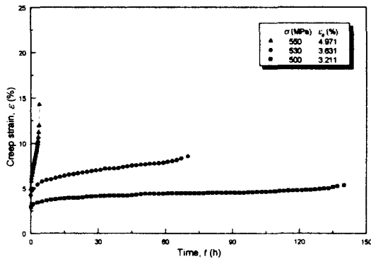
Fig. 2(a) Creep curves for friction welded joint (STD61-SCM440) at 400°C
