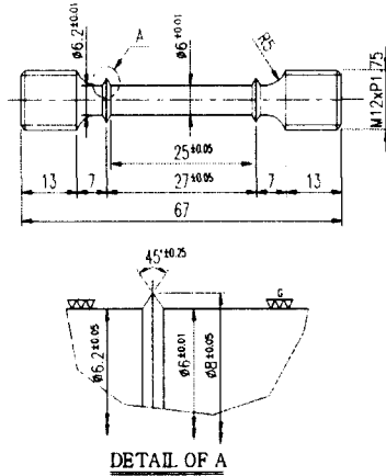
Fig. 1 Shape and dimension of creep test specimen
