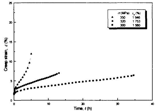
Fig. 2(b) Creep curves for friction welded joint (STD61-SCM440) at 500°C
