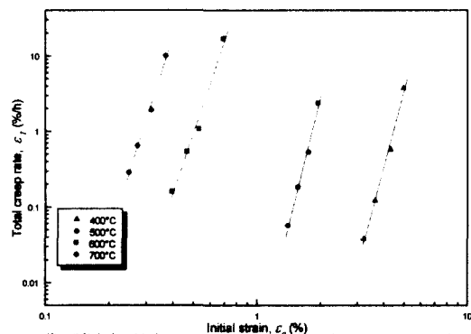
Fig. 6 Relationship between creep stress and steady state creep rate of STD61 to SCM440 at 400, 500, 600 and 700°C
