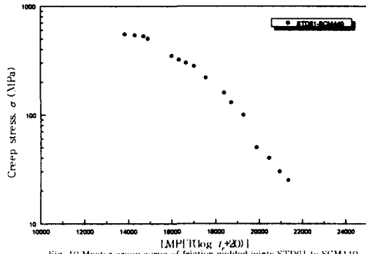
Fig. 10 Master creep curve of friction welded joints STD61 to SCM440 at 400, 500, 600 and 700°C
