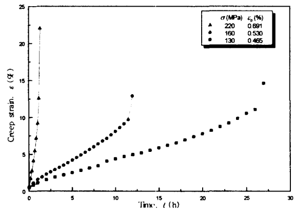
Fig. 2(c) Creep curves for friction welded joint (STD61-SCM440) at 600°C
