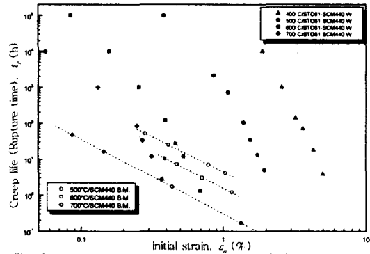
Fig. 9 Relationship between rupture time and initial strain for friction welded joints (STD61-SCM440) and SCM440 base metals at 400, 500, 600 and 700°C
