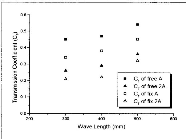
Fig 7. C_T vs Wave Length
