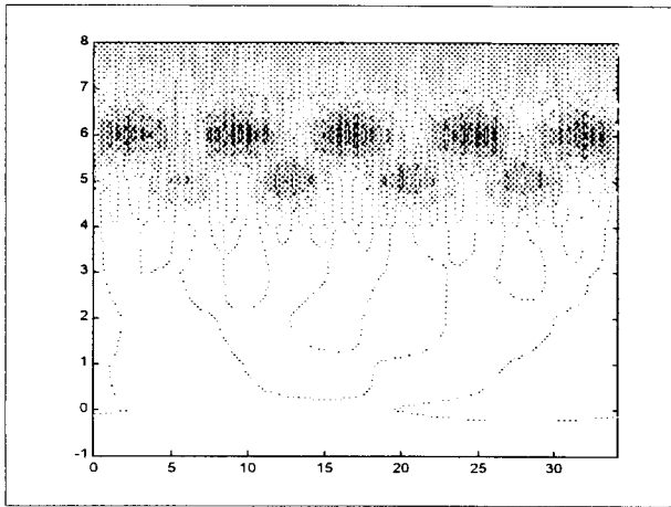
Fig 5. Wavelet Diagram of Fore Time History
