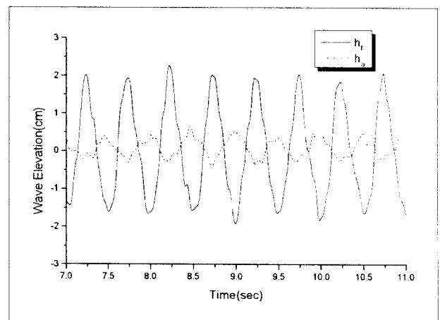
Fig 4. Time Histories of Up/Down Stream of Wave Absorber
