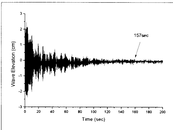
Fig 2. Time History of Wave Elevation W/O Wave Absorber
