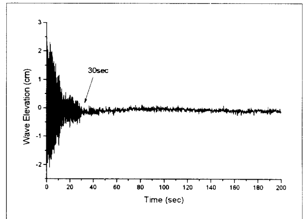
Fig 3. Time History of Wave Elevation W Wave Absorber
