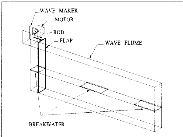
Fig 1. Experimental Sep Up
