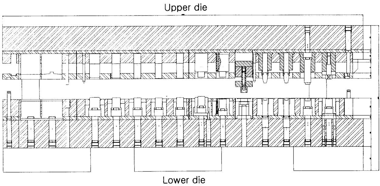
Fig.1 Die assembling drawing
