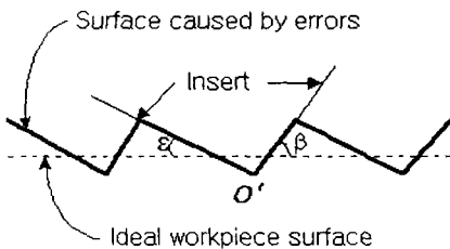
Fig. 4 Identification of the inclination angle of the insert from the machined surface
