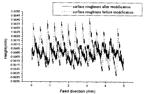
Fig. 6 Comparison of the surface roughness before and after the modification of the insert
