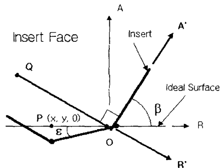
Fig. 5 Insert design for machining flat surface
