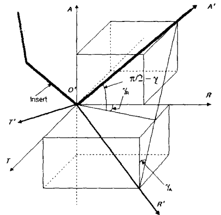
Fig. 2 The Relation between TRA and T'R'A' Coordinate
