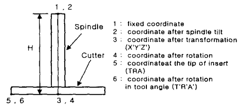
Fig. 1. Coordinate of the Machine Tool
