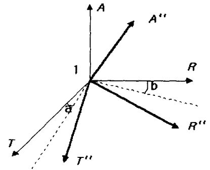
Fig. 3 Coordinate transformation considering spindle tilt
