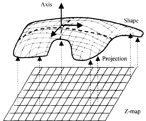
Fig.10 Creation of section curves using projection method of Z-map
