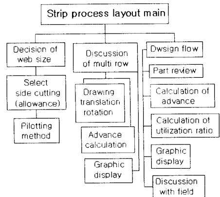
Fig. 8 Flow chart of strip process layout making procedure
