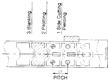
Fig.9 Strip process layout
