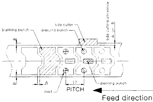
Fig.4 Web size on the strip process layout
